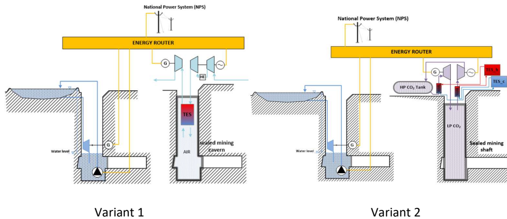
HESS operation diagram in two variants
