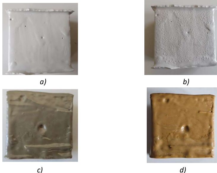
Sikagard® WallCoat T sample before test (a), sample after 180 days of exposure in acid solution (b), Sikagard® M 790 sample before test (c), sample after 180 days of exposure to acid solution (d).
