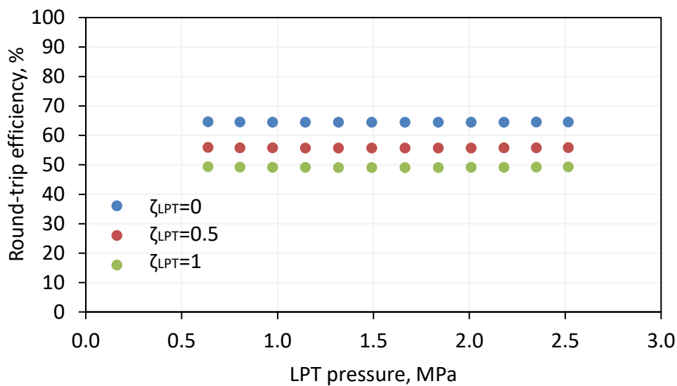
Fig. 36 Dependence of energy storage system efficiency on LPT tank pressure (Case 300 °C, \eta_{iC} = \eta_{iEx} = 80\% )
