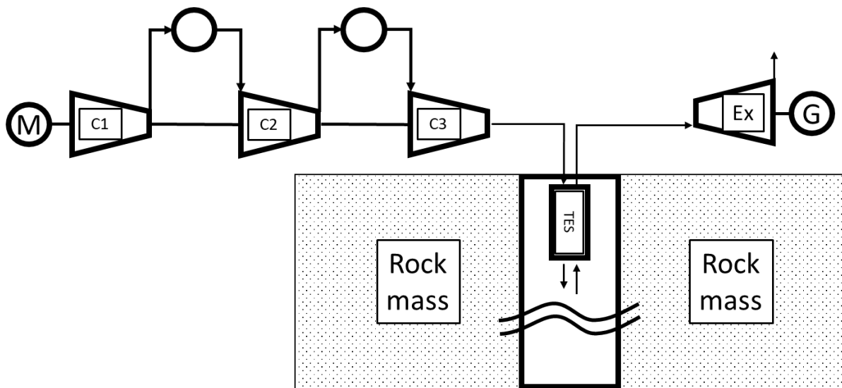
Fig. 5 Diagram of the analyzed adiabatic energy storage system in compressed air (CASE C)
