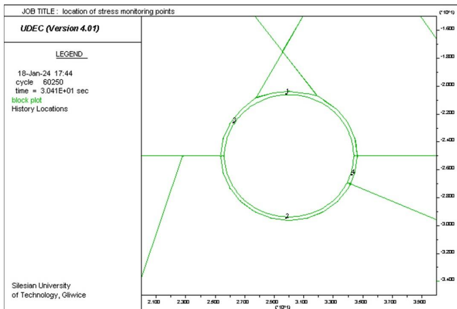
Fig. 11. Stress monitoring locations in the enclosure.
