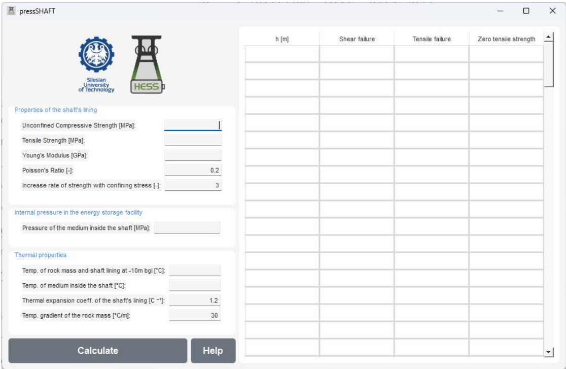
Fig. 17. Interface of app with data from real case scenario.
