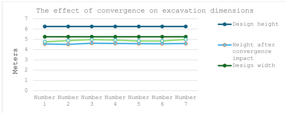
Fig. 8. Convergence of underground workings measured in the mine.
