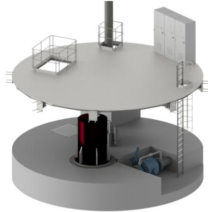
Fig. 7. Lower and upper levels of service platforms installed in the shaft
